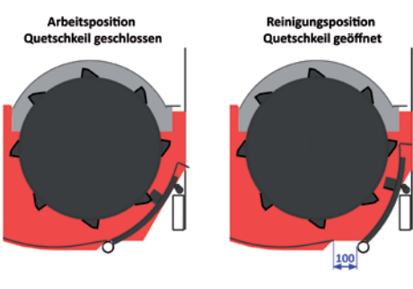
STONE SEPARATOR
